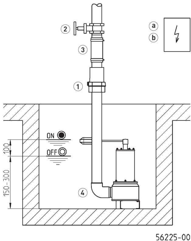
Installation example of feet
