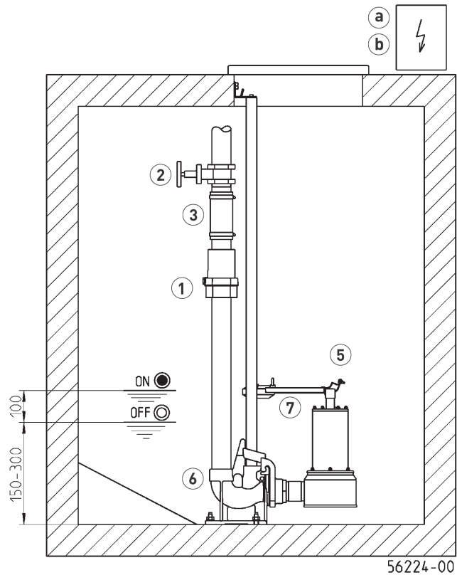
Installation example with sliding tube system
