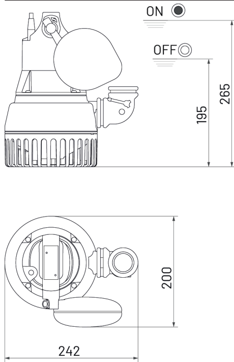
Dimensions and switching points float switch (mm)
