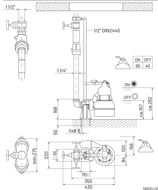
Dimensions and switching points GR 32 (mm)
